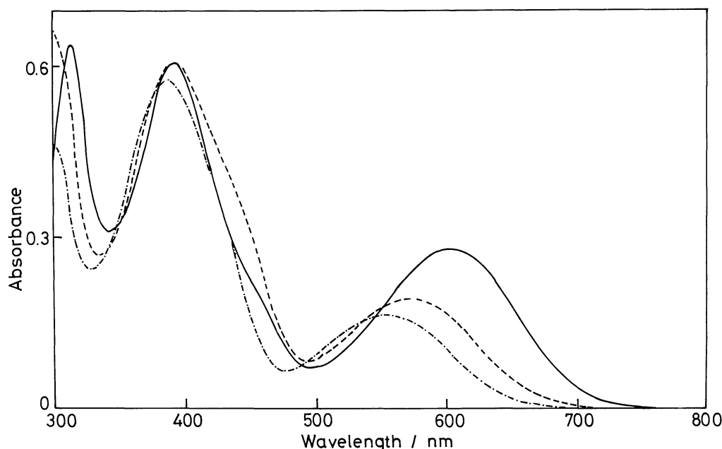
Fig. 3. Absorption spectra of 7a + 7b (total concentration, 1.0 \times 10^{-4} mol \text{dm}^{-3} ) at the photostationary state in hexane (---), in benzene (----), and in HMPA (—). Conversion from the open-ring to the closed-ring form was 39% in hexane, 44% in benzene, and 75% in HMPA. The absorption bands longer than 500 nm and at around 400 nm are ascribable to 7b , and shoulders at around 450 nm to 7a .
